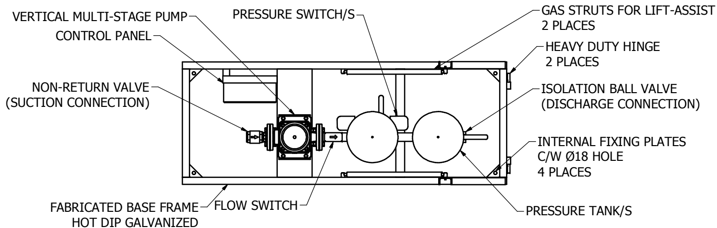
PUMPSET ASSEMBLY - PLAN VIEW (ENCLOSURE NOT SHOWN)
