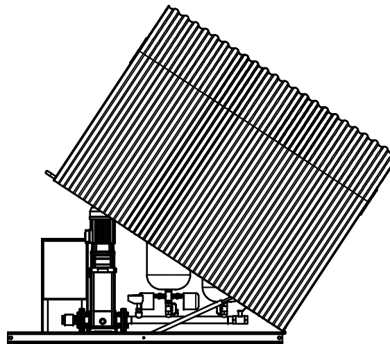
FULL ASSEMBLY - SIDE VIEW (PARTIALLY OPEN)
